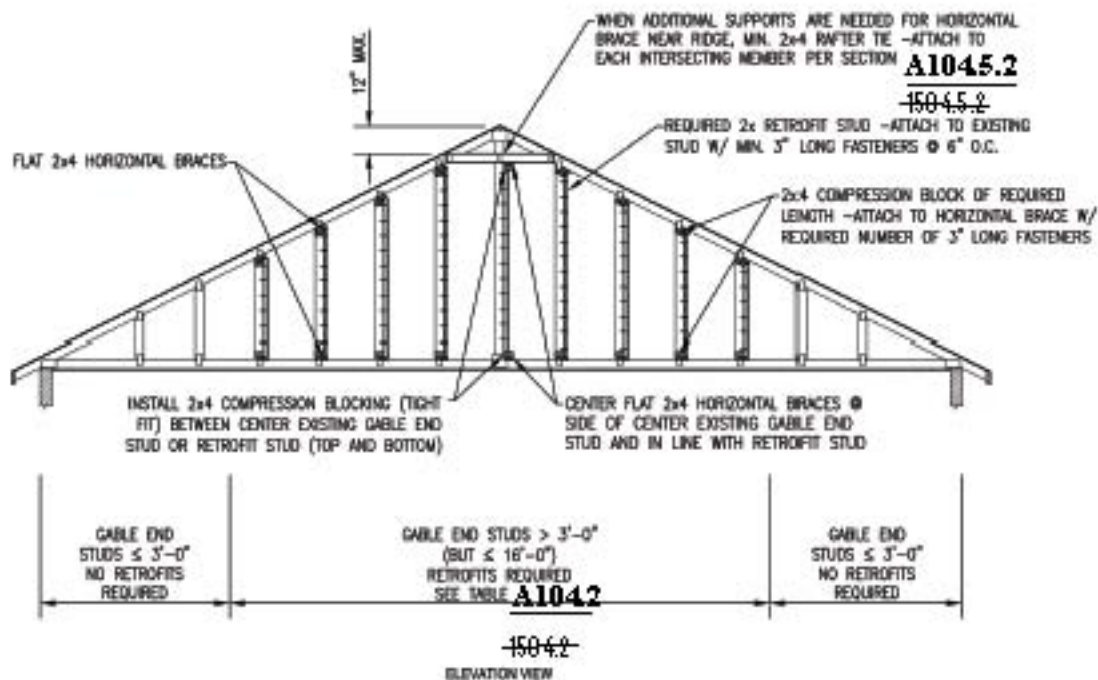
FIGURE A1045.2 DETAIL OF RETROFIT RIDGE TIE INSTALLATION
